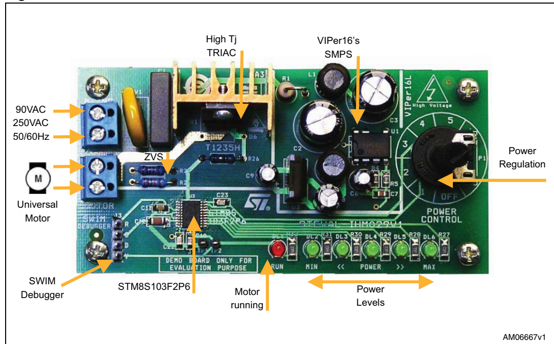
Figure 9. Demonstration board overview
