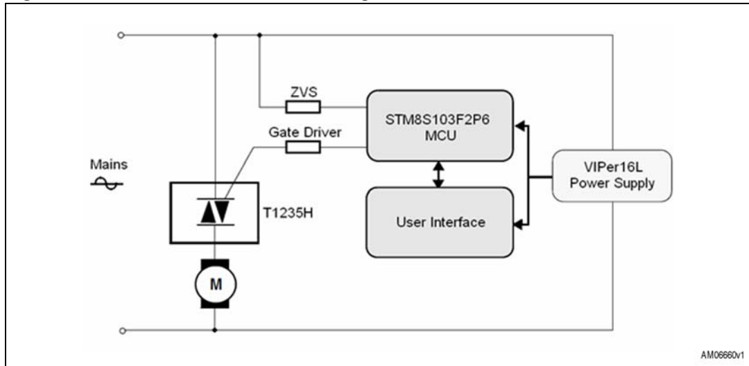
Figure 2. STEVAL-IHM029V1 block diagram
