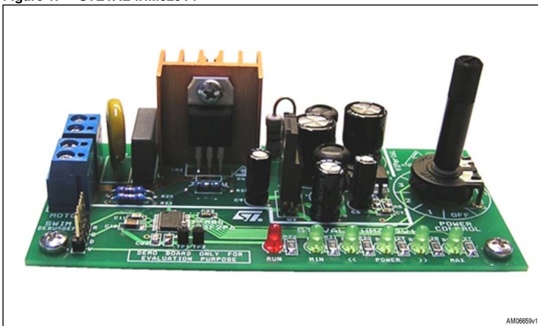
Figure 1. STEVAL-IHM029V1
