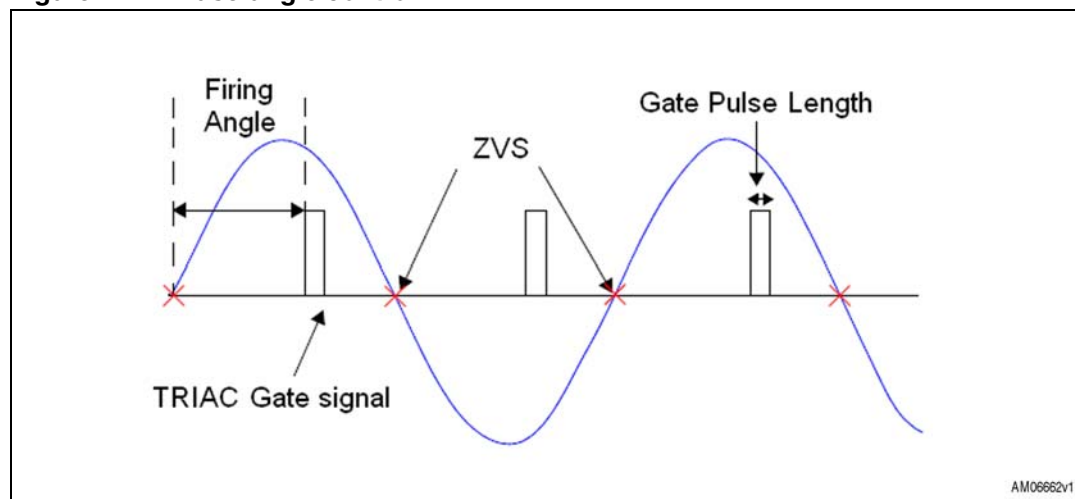
Figure 4. Phase-angle control
