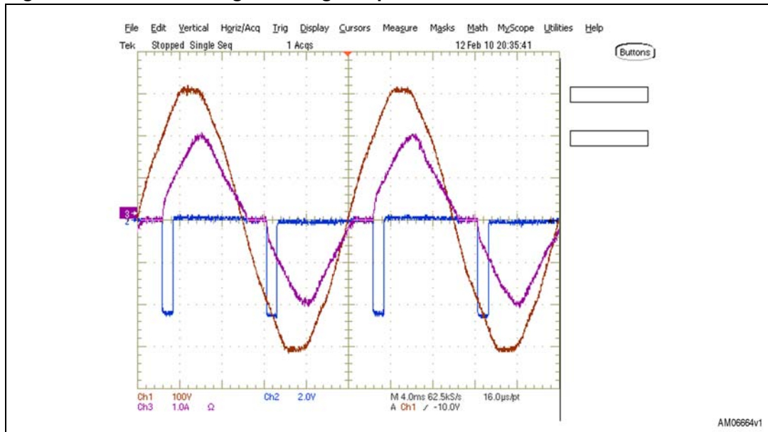
Figure 6. Motor working at the highest power level
