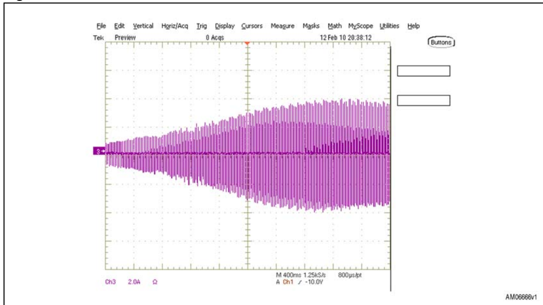
Figure 8. Soft-start
