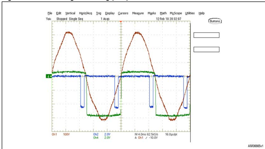
Figure 7. Zero-voltage switching (ZVS)
